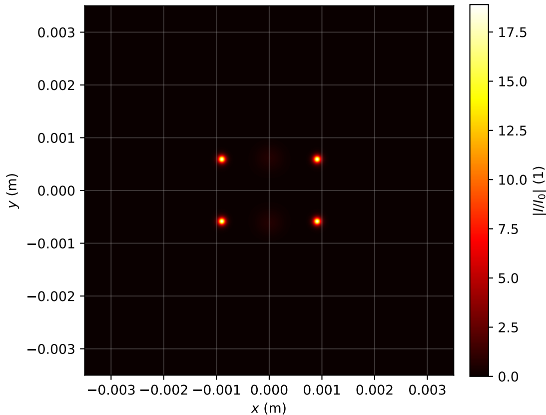
Intensity profile I(x, y, z = 1.115)/I_0 , P_{in}=5.0P_{cr} , artificial time
